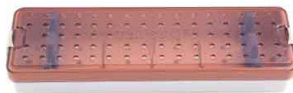
B0000.4 内窥镜消毒盒 For endoscope 255×71×36mm
